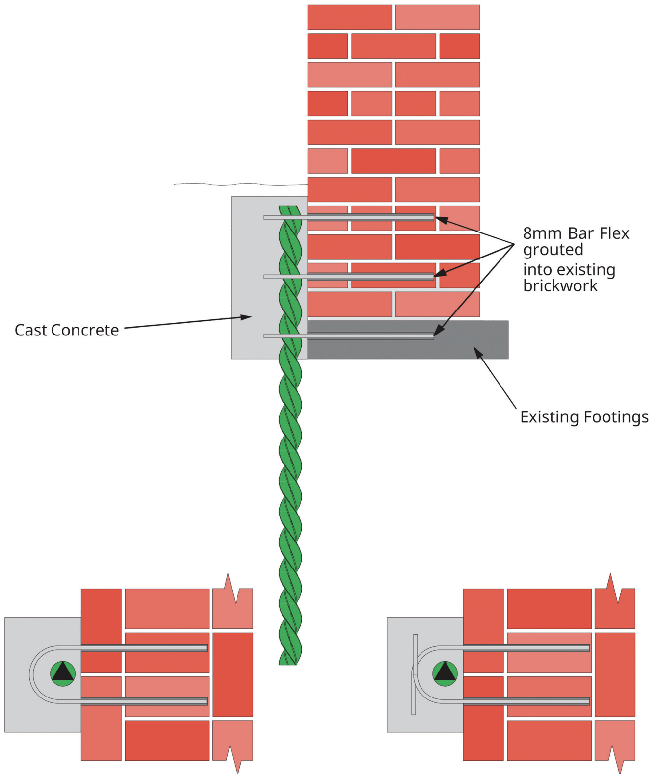
Plan Views
